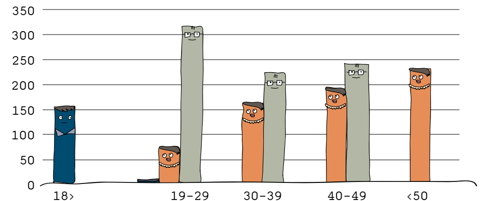
Age distribution
