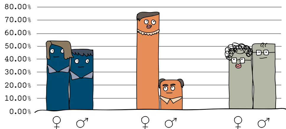
Gender distribution
